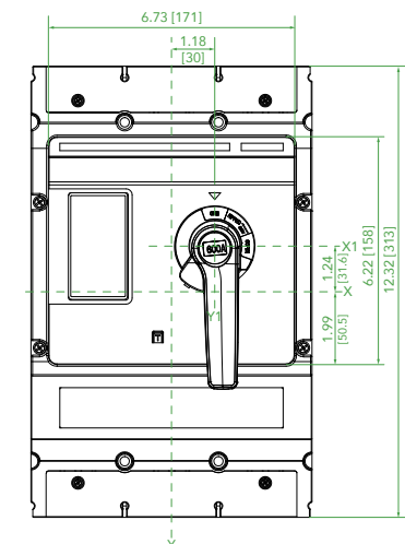
RHD24N Rotary Handle for M4 Unit: in [mm]
