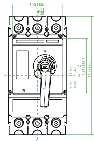
RHD23N Rotary Handle for M3 Unit: in [mm]
